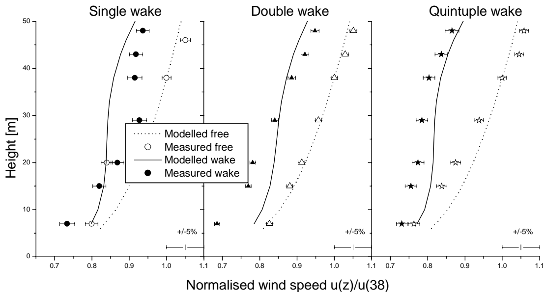
Figure 8: Vertical profiles of measured and modelled normalised wind speeds for the free and wake flow; Vindeby single(67 records), double (101) and quintuple (43) wakes, stable stratification, 6% turbulence intensity, 5\text{ms}^{-1} (single) and 7.5\text{ms}^{-1} (double and quintuple) mean wind speed; error bars indicate the standard errors
