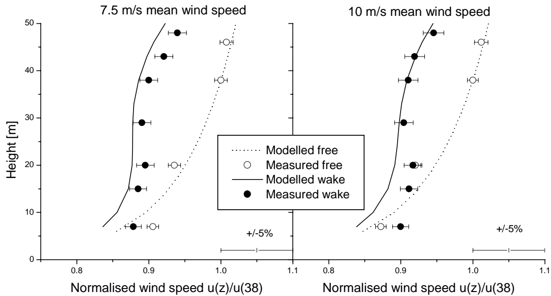
Figure 5: Vertical profiles of measured and modelled normalised wind speeds for the free and wake flow; Vindeby single wake with wind direction 18^\circ - 28^\circ , near-neutral stability, 6% turbulence intensity, 7.5 \text{ ms}^{-1} (170 records) and 10 \text{ ms}^{-1} (59) mean wind speed; error bars indicate the standard errors
