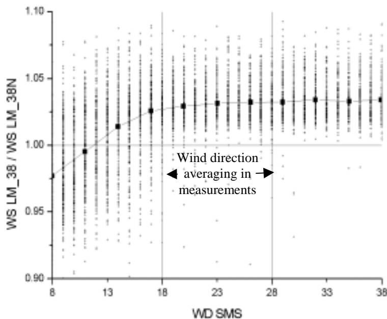
Figure 2: Ratio between the wind speeds (WS) measured by the north and south anemometer at 38 m height the LM versus wind direction (WD) measured at the SMS
