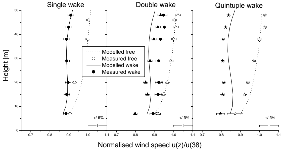
Figure 9: Vertical profiles of measured and modelled normalised wind speeds for the free and wake flow; Vindeby single (86 records), double (65) and quintuple (275) wakes, unstable stratification, 6% turbulence intensity, 7.5\text{ms}^{-1} mean wind speed; error bars indicate the standard errors
