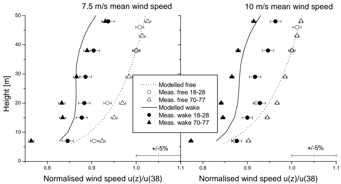
Figure 6: Vertical profiles of measured and modelled normalised wind speeds for the free and wake flow; Vindeby double wake with wind direction 70^\circ\text{-}78^\circ and 18^\circ\text{-}28^\circ , near-neutral stability, 6% turbulence intensity, 7.5\text{ms}^{-1} (18-28: 170 records; 70-77: 254) and 10\text{ms}^{-1} (18-28: 59; 70-77: 332) mean wind speed; error bars indicate the standard errors
