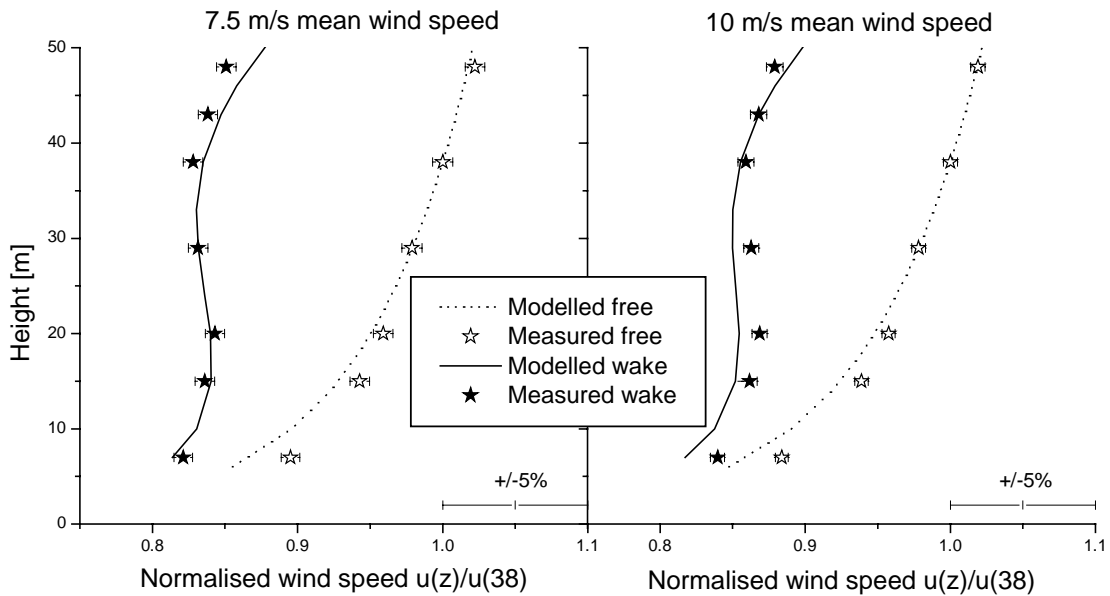
Figure 7: Vertical profiles of measured and modelled normalised wind speeds for the free and wake flow; Vindeby quintuple wake with wind direction 314^\circ\text{-}323^\circ , near-neutral stability, 6% turbulence intensity, 7.5\text{ms}^{-1} (420 records) and 10\text{ms}^{-1} (344) mean wind speed; error bars indicate the standard errors
