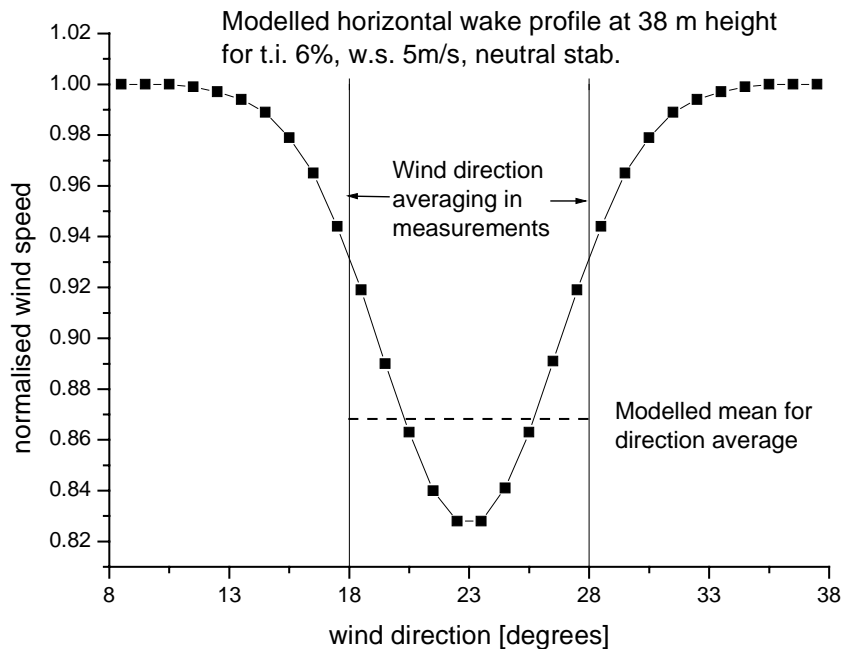
Figure 4: Wind direction dependent (horizontal) wake modelling at hub height for the case of 6% turbulence intensity, neutral atmospheric stability and a wind speed of 5 \text{ ms}^{-1} ; the dashed line shows the average for the wind direction sector 18^\circ to 28^\circ
