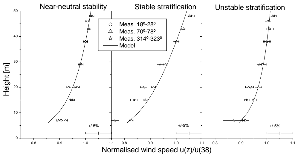
Figure 3: Measured and modelled free vertical wind speed profile for near neutral stratification ( |L| > 1000 ) (left), stable stratification ( 0 < L < 1000 ) (middle) and unstable stratification ( 0 > L > -1000 ); turbulence intensity bin 6% (5-7%), wind speed bin 7.5 \text{ ms}^{-1} ( 6-9 \text{ ms}^{-1} ), wind direction sectors as used for wake comparisons; error bars indicate the standard errors
