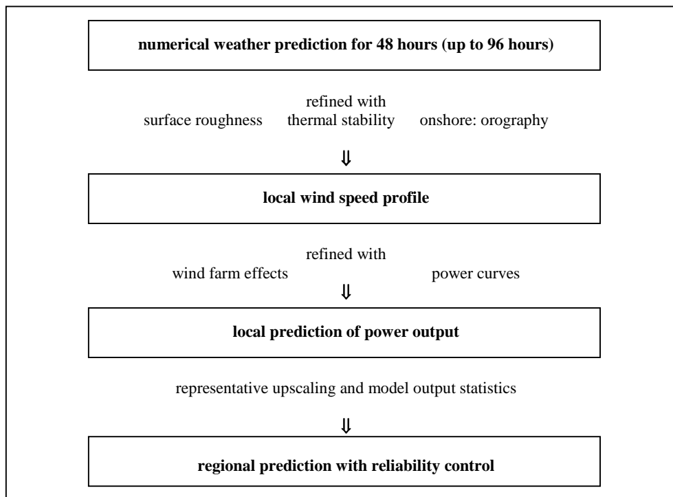
Figure 2: Principle of the prediction system Previento with a spatial refinement of the numerical weather prediction leading to a local prediction of power output at one site, subsequently used for regional upscaling
