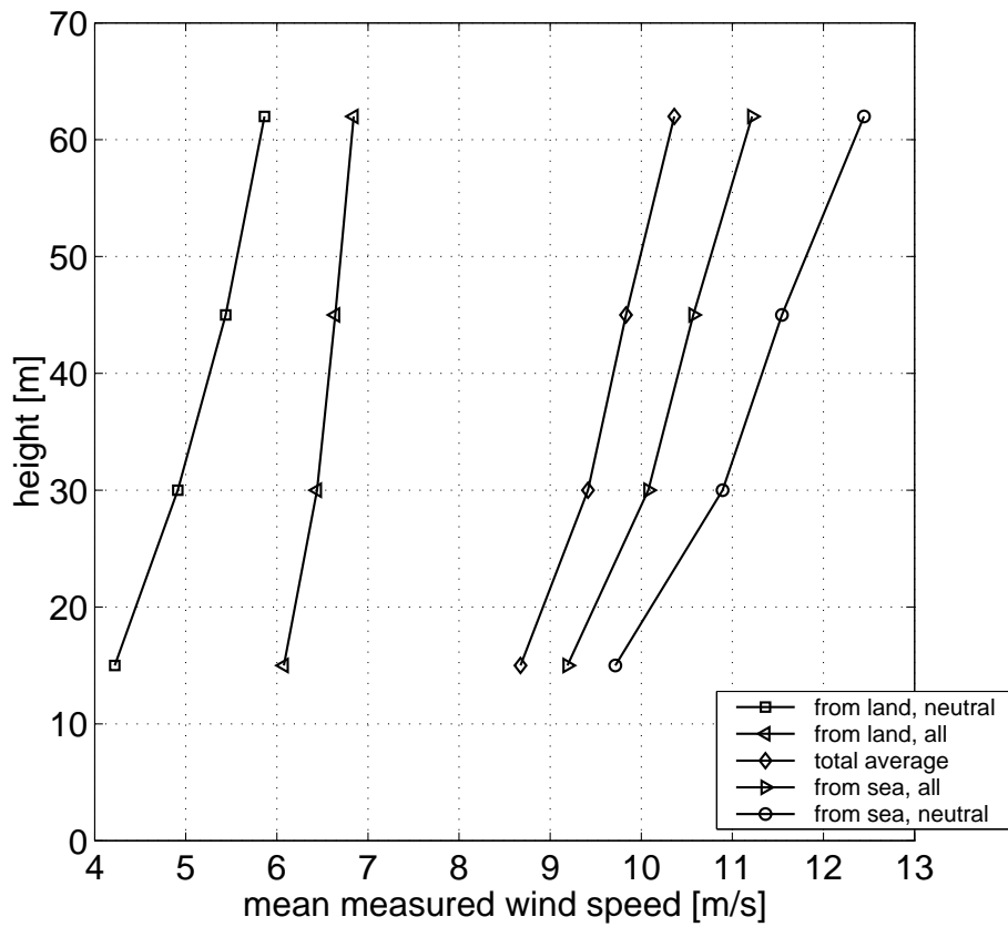
Figure 13: Mean profiles of wind speed; blowing from land to sea, from all directions and from sea to land. Neutral profiles have no difference in potential temperatures in 55m and 13m height. Sea-wind speeds in 62m exceed logarithmically extrapolated values. Winter period 10/2001 till 04/2002; Top: Lognormal scale, Bottom: linear scale
