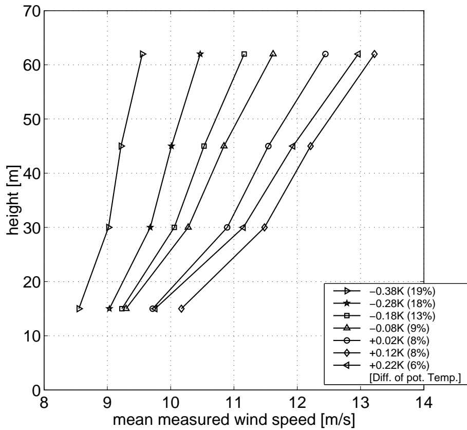
Figure 14: Sea-wind speed profiles depending on potential temperature difference [T55-T13+0.4K] . Frequency of occurrence in brackets. The wind speeds in 62m exceeding the logarithmic extrapolation seem to follow an almost linear increase. Winter period 10/2001 till 04/2002; Top: Lognormal scale, Bottom: linear scale
