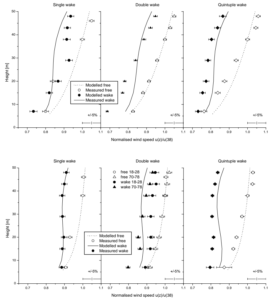
Figure 3: Vertical profiles of measured and modelled normalised wind speeds for the free and wake flow; Vindeby single, double and quintuple wakes, stable (top figure) and unstable (bottom figure) stratification, 6% turbulence intensity, 7.5m/s mean wind speed (except single wake stable: 5m/s); error bars indicate the standard errors
