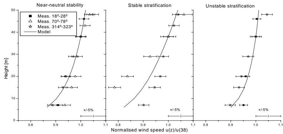
Figure 4: Measured and modelled free vertical wind speed profile for near neutral stratification ( |L| > 1000 ) (left), stable stratification ( 0 < L < 1000 ) (middle) and unstable stratification ( 0 > L > -1000 ); turbulence intensity bin 8% (7-9%), wind speed bin 5ms-1 (4-6ms-1), wind direction sectors as used for wake comparisons; error bars indicate the standard errors
