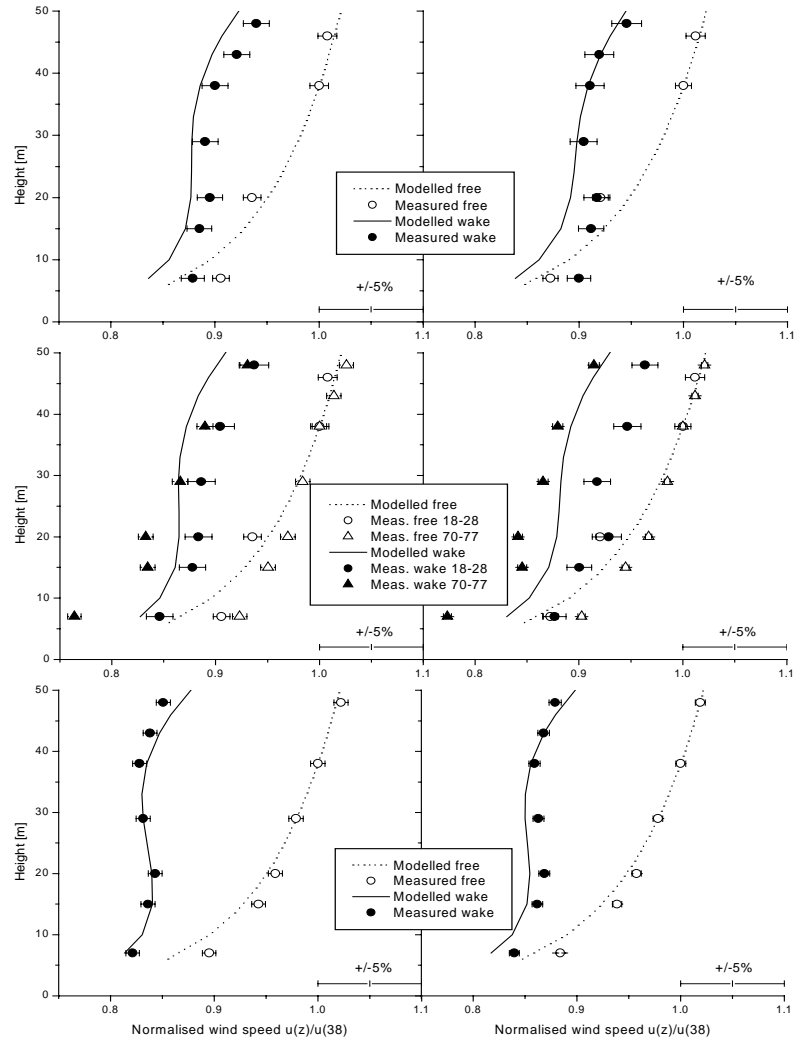
Figure 2: Vertical profiles of measured and modelled normalised wind speeds for the free and wake flow; Vindeby single (top figure), double (middle figure) and quintuple (bottom figure) wake with wind direction 314^\circ - 323^\circ , near-neutral stability, 6% turbulence intensity, 7.5m/s (left) and 10m/s (right) mean wind speed; error bars indicate the standard errors
